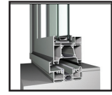
Double Weather Seal 23-44mm
