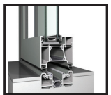
Low Threshold 9-30mm
